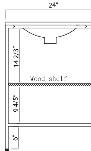
BACK VIEW
